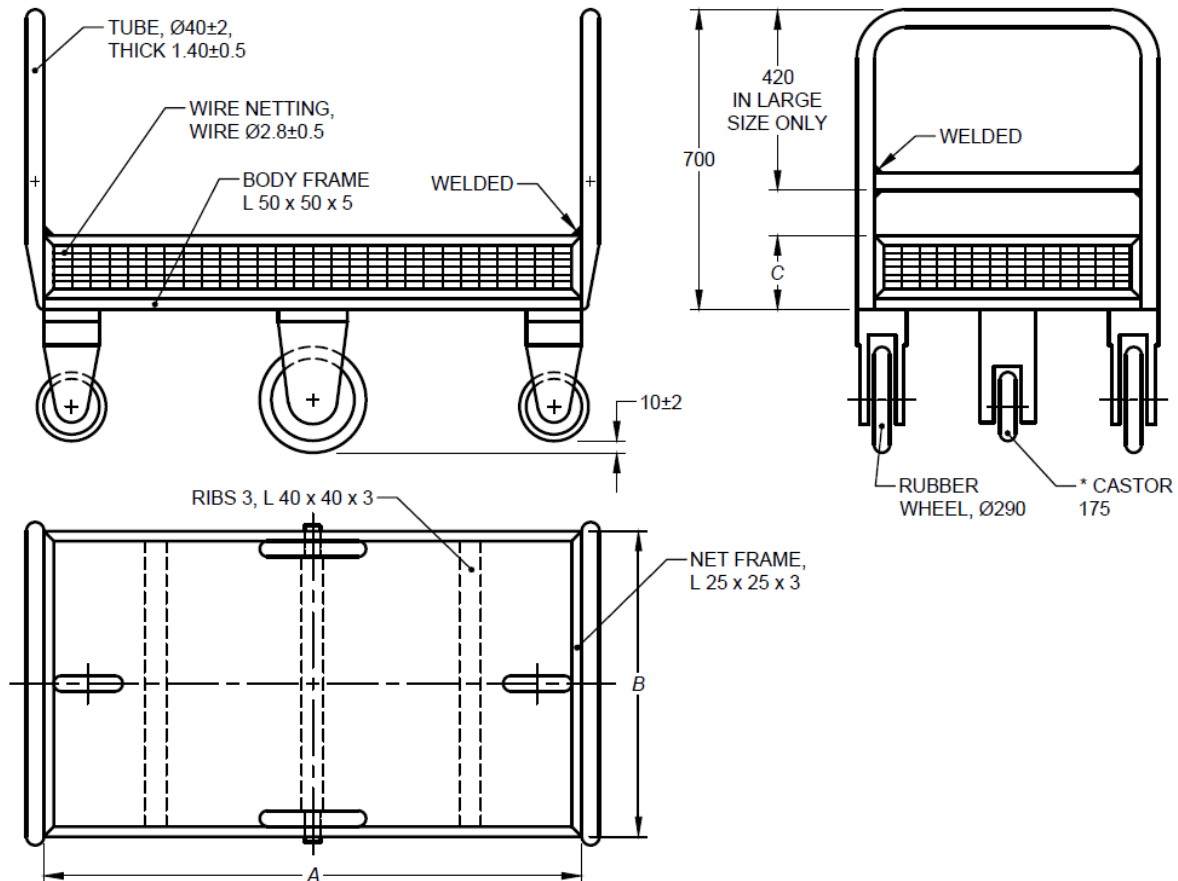
Fig. 1 MEDICAL STORE TROLLEY
